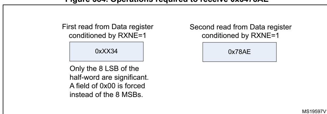
Figure 384. Operations required to receive 0x3478AE
