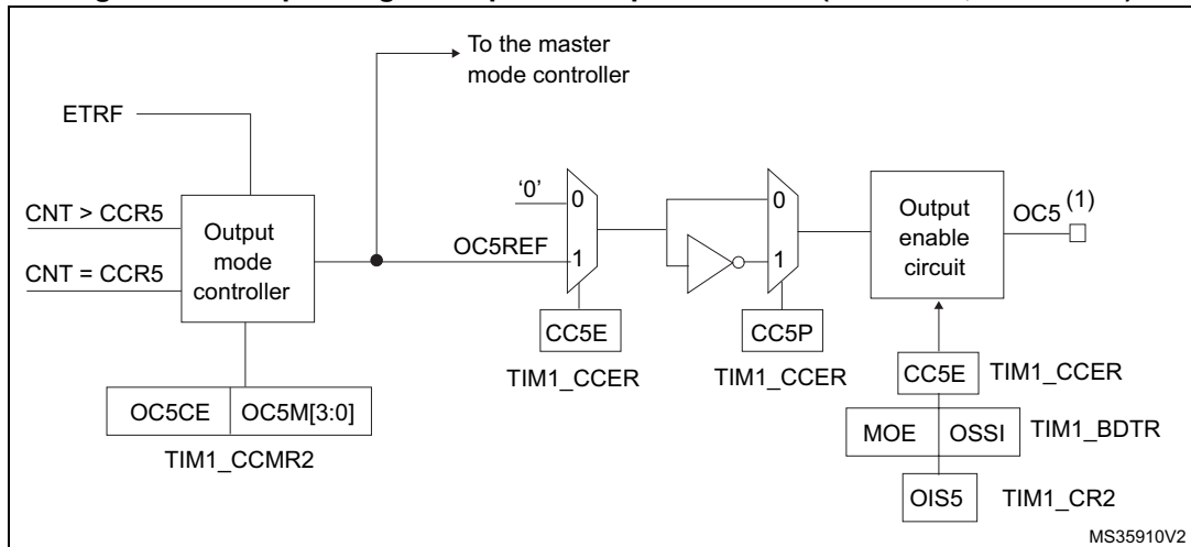
Figure 176. Output stage of capture/compare channel (channel 5, idem ch. 6)
