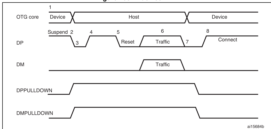
Figure 485. B-device HNP
