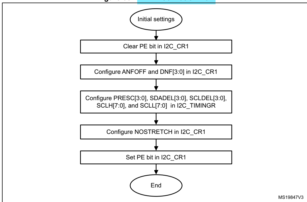
Figure 302. I2C initialization flow
